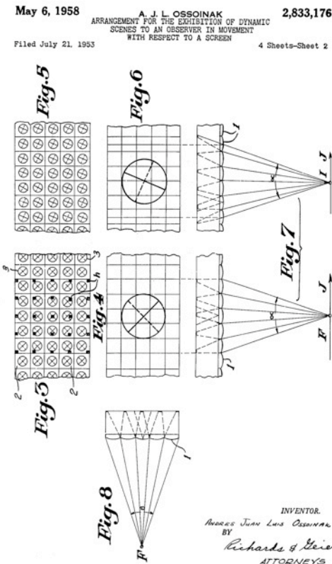
Figure 18: Integral lens array animation effects, U.S. Patent 2,833,176; Ossoinak 1958 (67).
