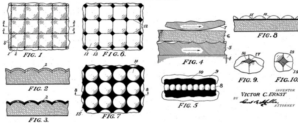
Figure 16: Full tone reproducing screen , U.S. Patent 1,991,888; Ernst 1935 (39).
