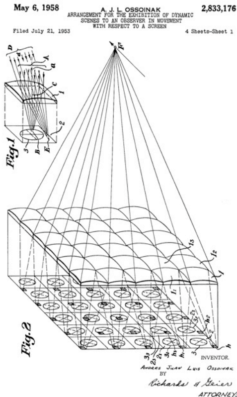
Figure 18: Integral lens array animation effects, U.S. Patent 2,833,176; Ossoinak 1958 (67).
