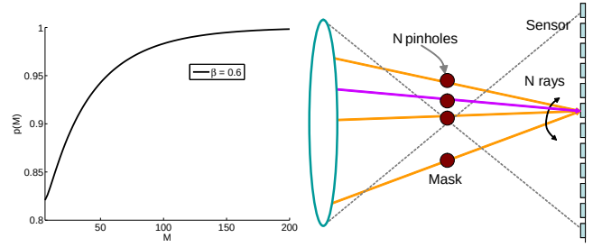
Figure 14: (Left) Plot showing the probability that at least 50% of the sensor pixels are not corrupted by glare as a function of the number of pixels within each tile for \beta = 0.6 . (Right) Multiple pinholes contribute to a single pixel if the spacing between the pinholes is reduced.
