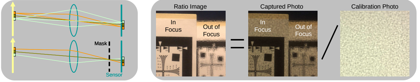
Figure 6: Recovering a full resolution image. (Left) Without mask, three scene patches create a focused image. With mask, for scene parts in focus, at least a subset of rays reach the sensor, creating the same (but less bright) image of the three scene patches. (Right) By dividing the captured photo with a calibration photo, we can recover the scene parts in focus at full resolution. Out of focus scene parts, however, exhibit aliasing as shown by the resolution chart in the back.
