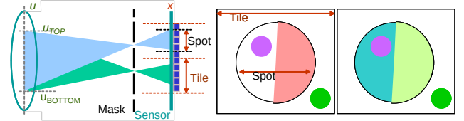
Figure 7: Capturing a photo by placing a pinhole mask near the sensor. ‘Tile’ refers to the maximum size of the non-overlapping aperture image formed by a single pinhole. For small apertures ( u_{top} \leftrightarrow u_{bottom} ), the image of the aperture is restricted to a ‘spot’ within the tile. (Middle) An orange colored vertically striped object is focused on the sensor. The purple dot indicates an outlier corresponding to the reflection glare. (Right) Scatter-glare (cyan) creates bias making the orange colored scene object look more greenish. Body glare (green dot) is contributed from a ray outside the view cone towards the aperture.
