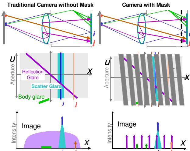
Figure 4: Comparison of glare formation in ray-space and sensor image for a traditional camera and our mask based camera. A focused blue scene patch could contribute to scattering (cyan), reflection (purple) and body glare (green). Since the sensor image is a projection of the ray-space along angular dimensions, the sum of these components creates a low frequency glare for a traditional camera. However, by inserting a high frequency occluder (gray), in front of the sensor, these components are converted into a high frequency 2D pattern and can be separated.
